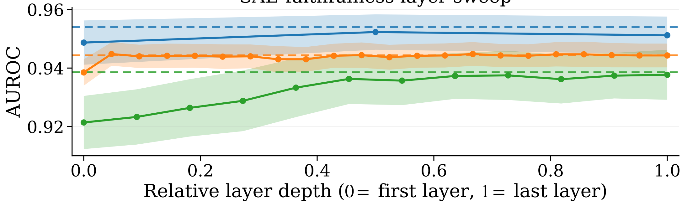
SAE-faithfulness layer sweep
